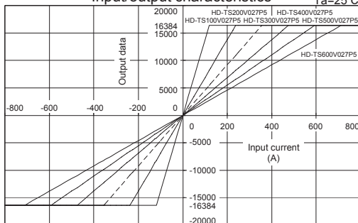
Input/output characteristics
