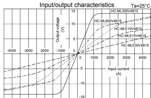
Input/output characteristics
